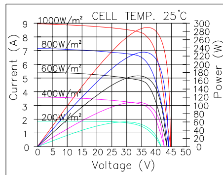
Characteristics Curve
